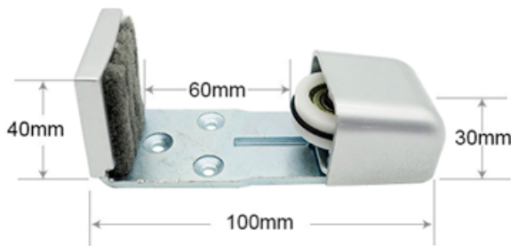
Large brush swing stopper
