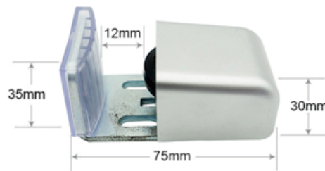
Small rubber swing stop
